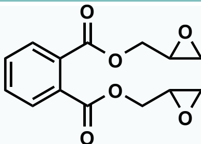
Diglycidyl o-Phthalate
