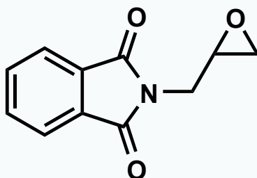
N-Glycidyl Phthalate
